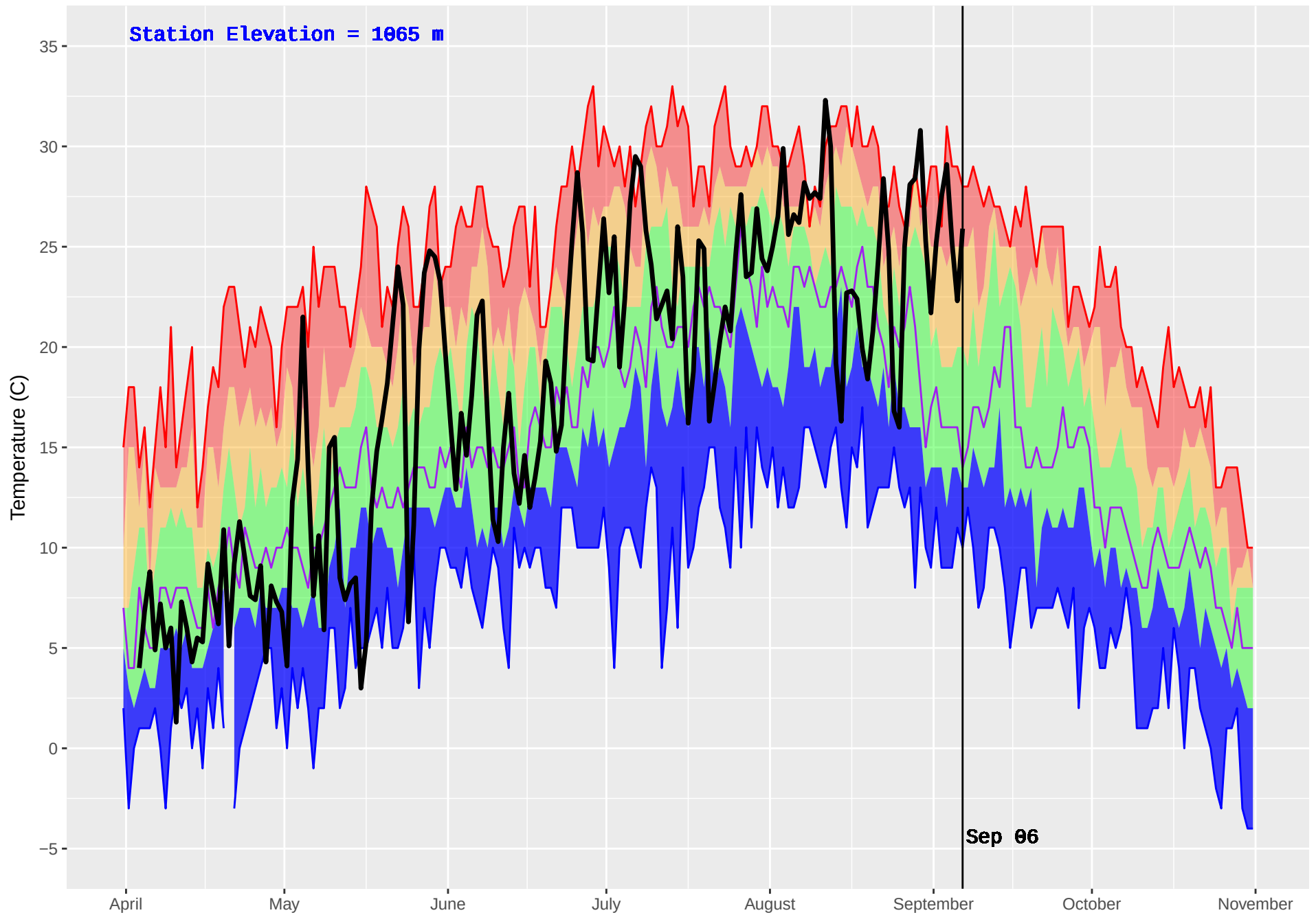
ASPEN GROVE (302) : Historical (1998–2016) and Current (2017) Noon Temperature
