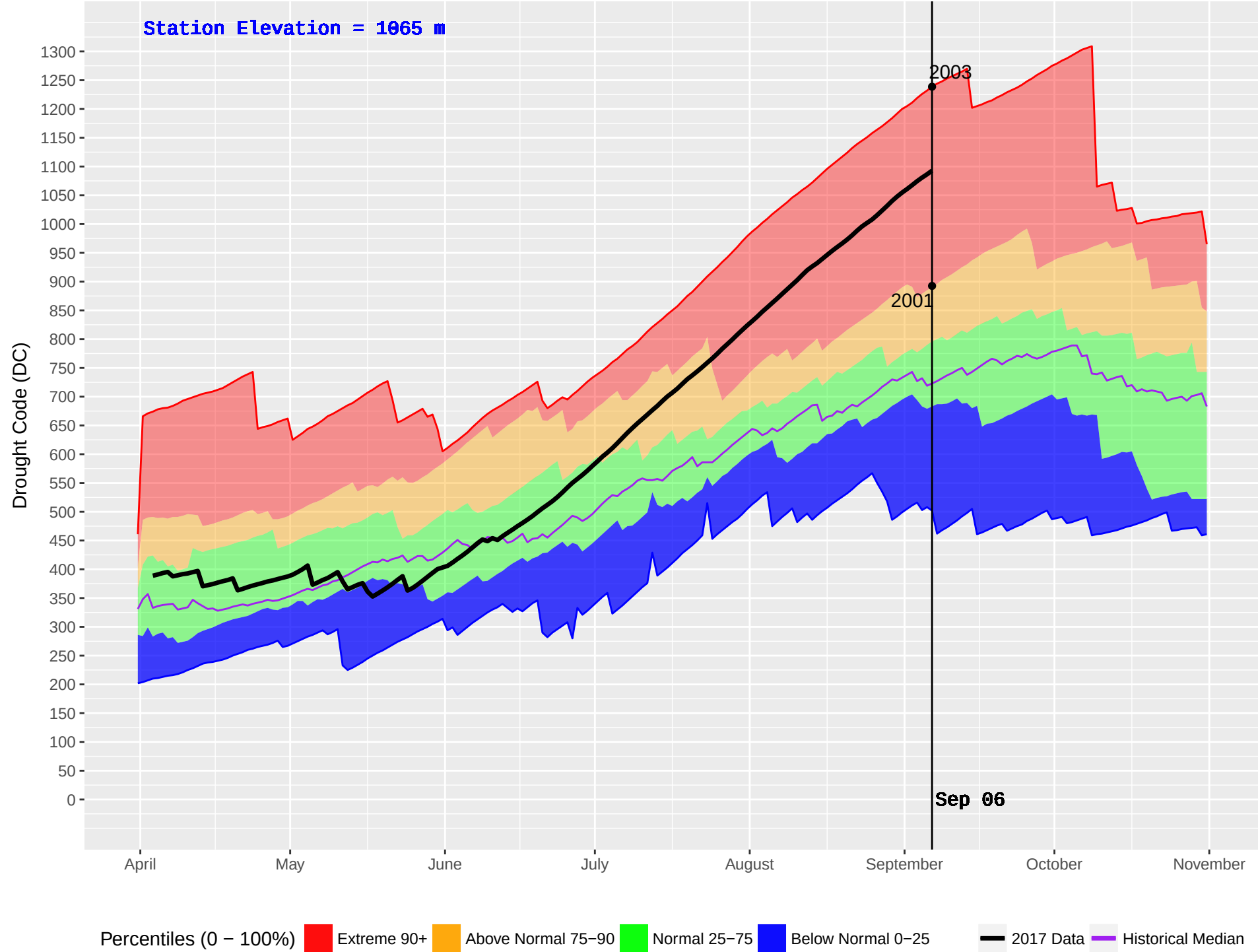
ASPEN GROVE (302) : Historical (1998–2016) and Current (2017) Noon Drought Code (DC)
